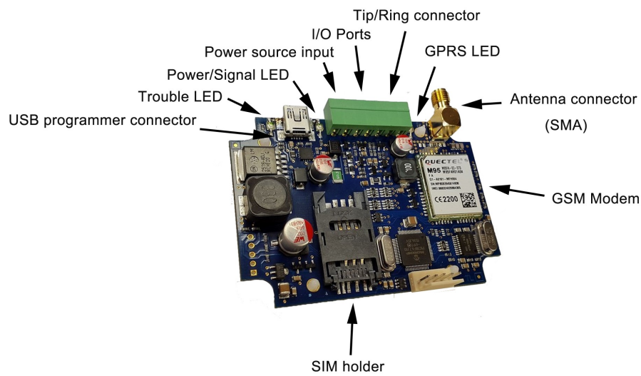
Figure 1: the buildup of the module
