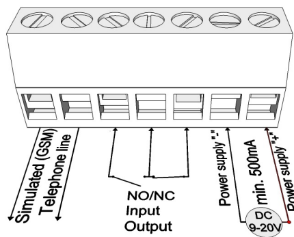
Figure 2: Series diaram wiring terminal
