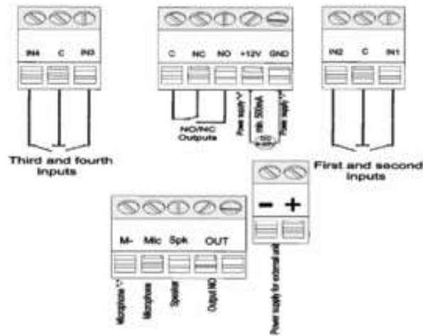
Figure 3: wiring diagram
